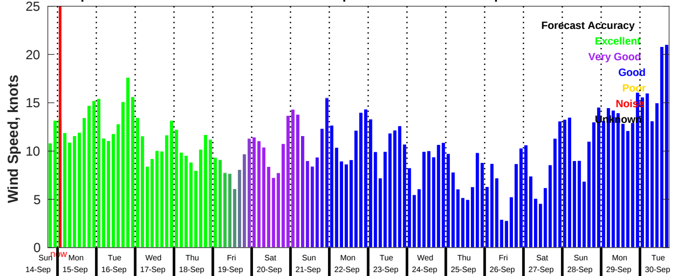
GFS Wind Speed Forecast for NDBC 42020 from 14-Sep-2025 18:00:00 to 30-Sep-2025 18:00:00
