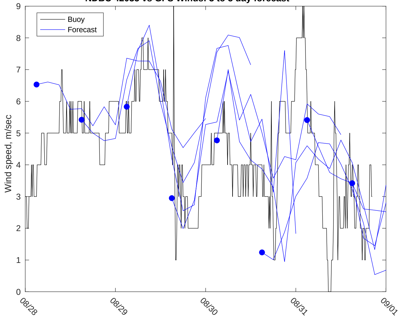
NDBC 42035 vs GFS Winds: 3 to 5 day forecast
