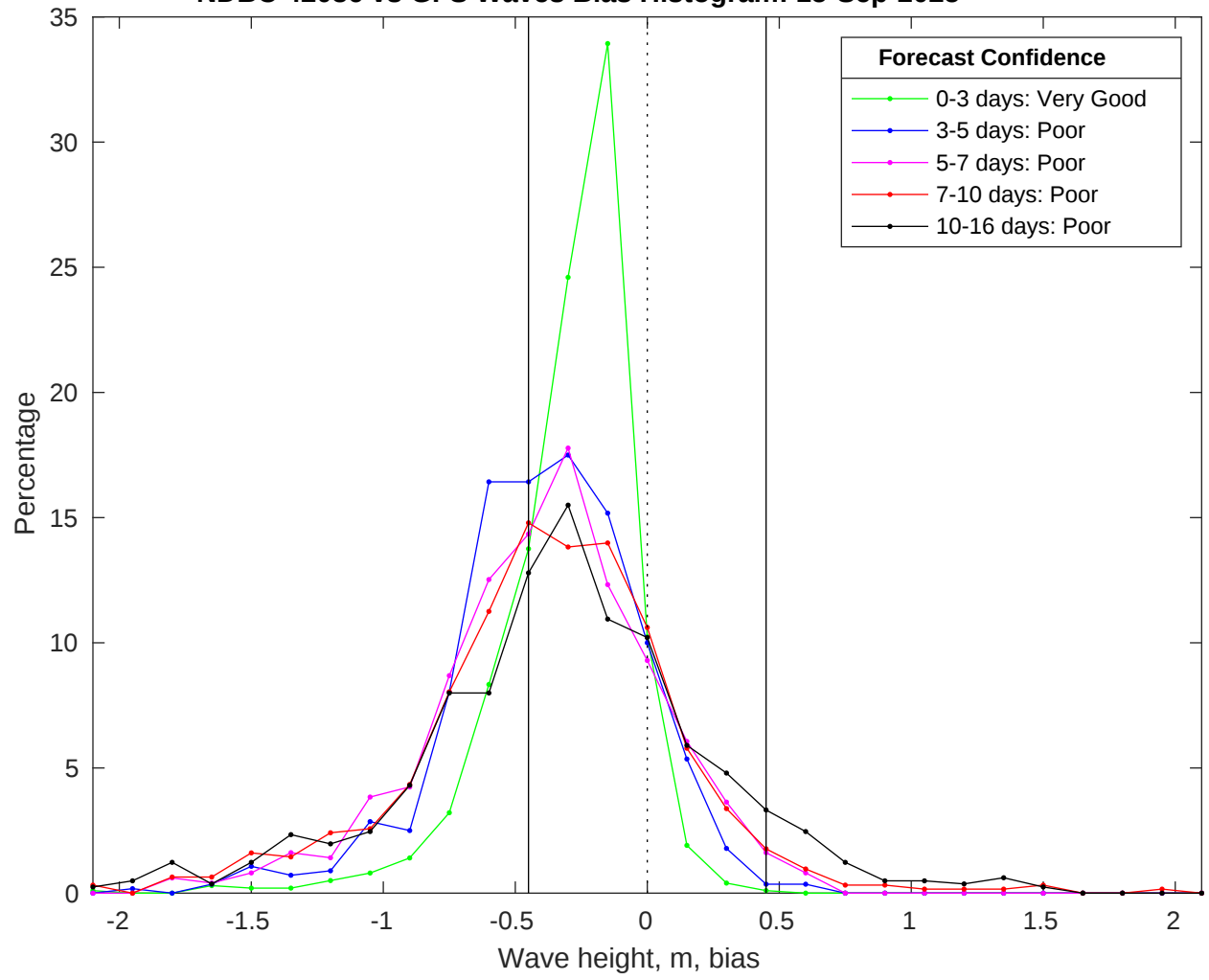
NDBC 42036 vs GFS Waves Bias Histogram: 15-Sep-2025
