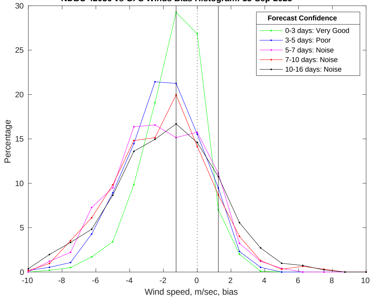
NDBC 42036 vs GFS Winds Bias Histogram: 15-Sep-2025
