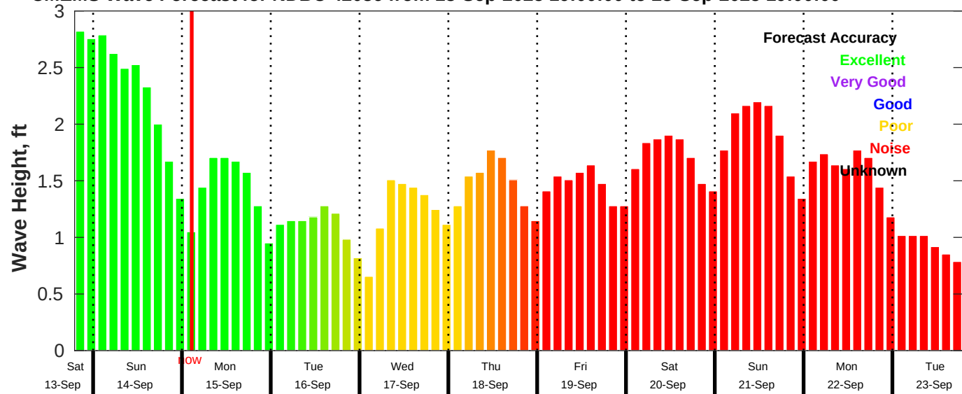
CMEMS Wave Forecast for NDBC 42036 from 13-Sep-2025 19:00:00 to 23-Sep-2025 19:00:00
