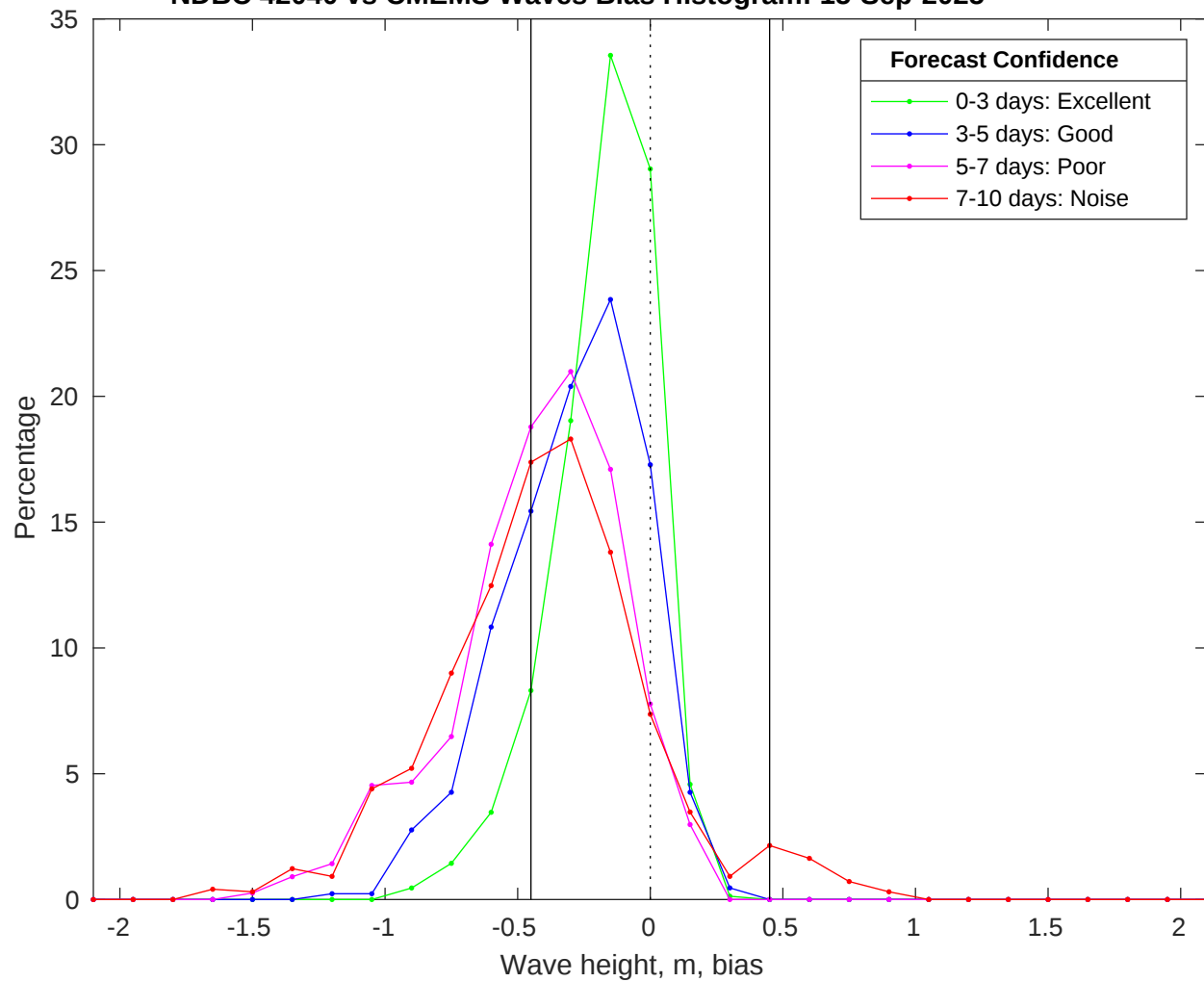
NDBC 42040 vs CMEMS Waves Bias Histogram: 15-Sep-2025
