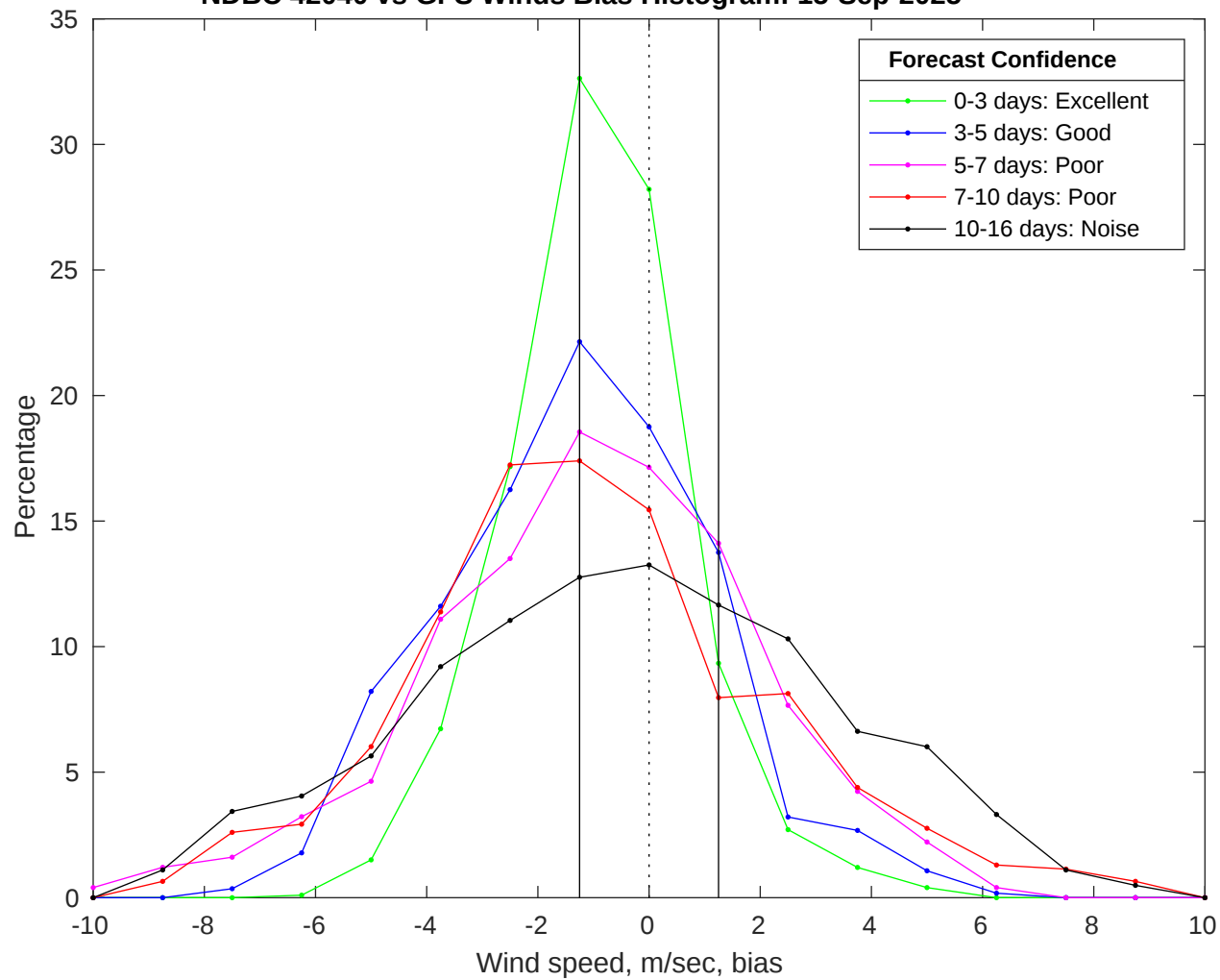
NDBC 42040 vs GFS Winds Bias Histogram: 15-Sep-2025
