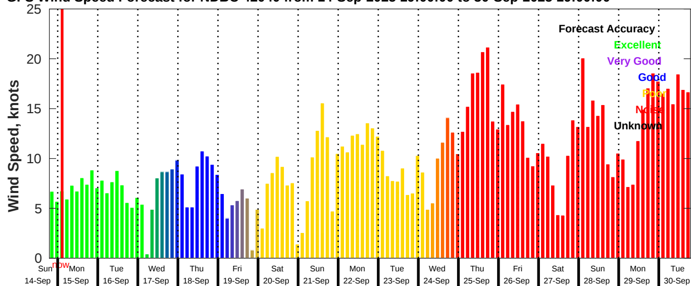
GFS Wind Speed Forecast for NDBC 42040 from 14-Sep-2025 19:00:00 to 30-Sep-2025 19:00:00
