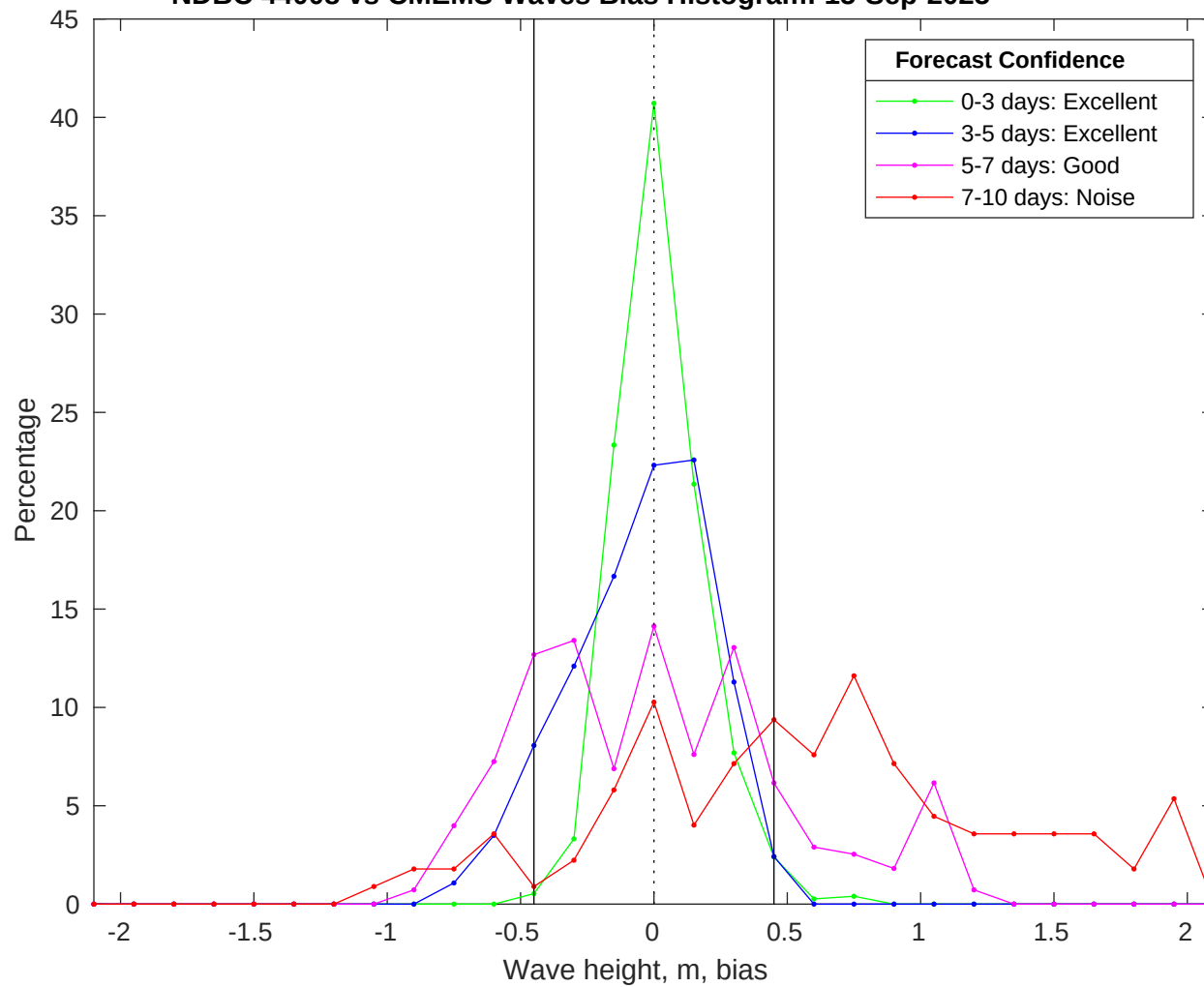
NDBC 44008 vs CMEMS Waves Bias Histogram: 15-Sep-2025
