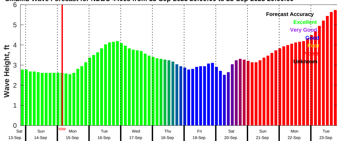
CMEMS Wave Forecast for NDBC 44008 from 13-Sep-2025 20:00:00 to 23-Sep-2025 20:00:00
