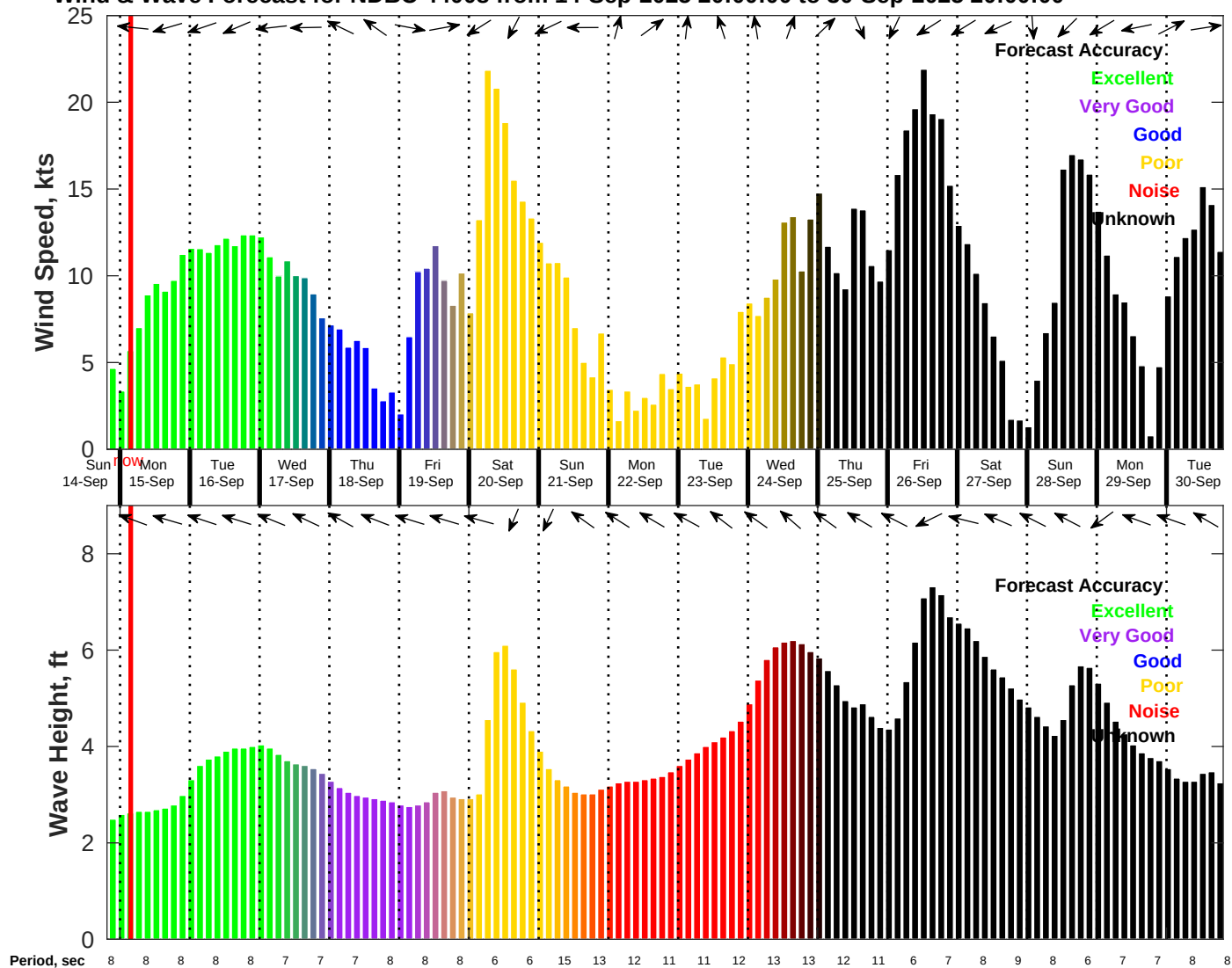
Wind & Wave Forecast for NDBC 44008 from 14-Sep-2025 20:00:00 to 30-Sep-2025 20:00:00
