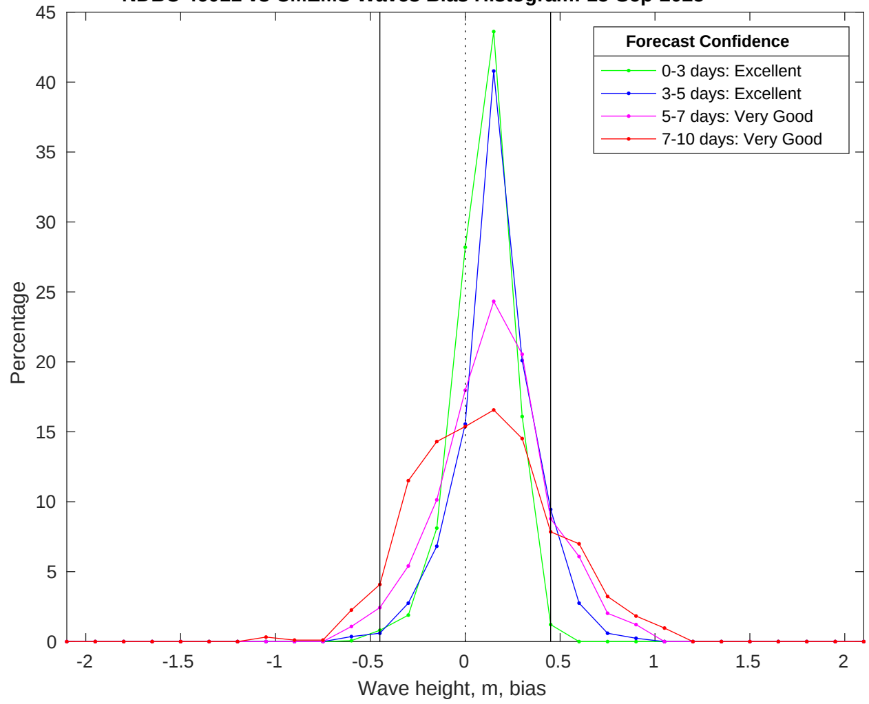
NDBC 46011 vs CMEMS Waves Bias Histogram: 15-Sep-2025
