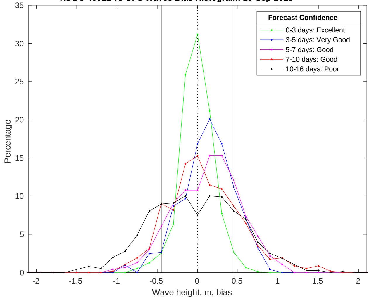
NDBC 46011 vs GFS Waves Bias Histogram: 15-Sep-2025
