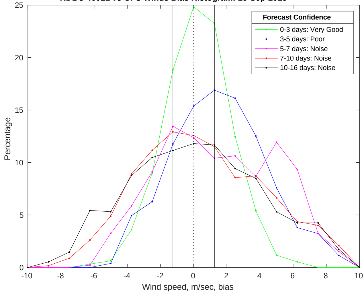
NDBC 46011 vs GFS Winds Bias Histogram: 15-Sep-2025
