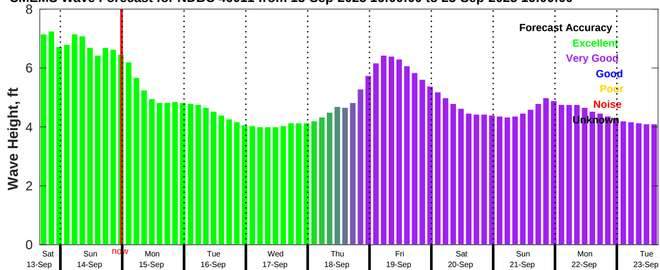
CMEMS Wave Forecast for NDBC 46011 from 13-Sep-2025 16:00:00 to 23-Sep-2025 16:00:00
