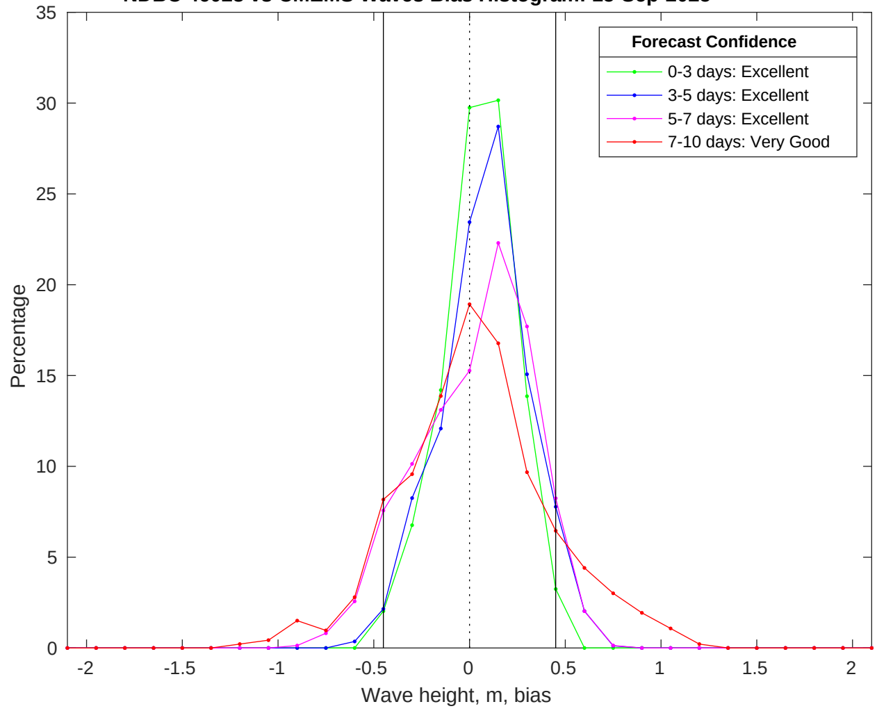
NDBC 46028 vs CMEMS Waves Bias Histogram: 15-Sep-2025
