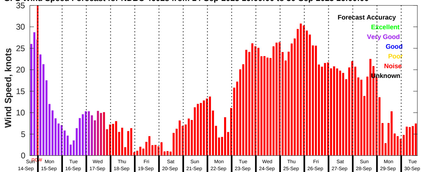
GFS Wind Speed Forecast for NDBC 46028 from 14-Sep-2025 16:00:00 to 30-Sep-2025 16:00:00
