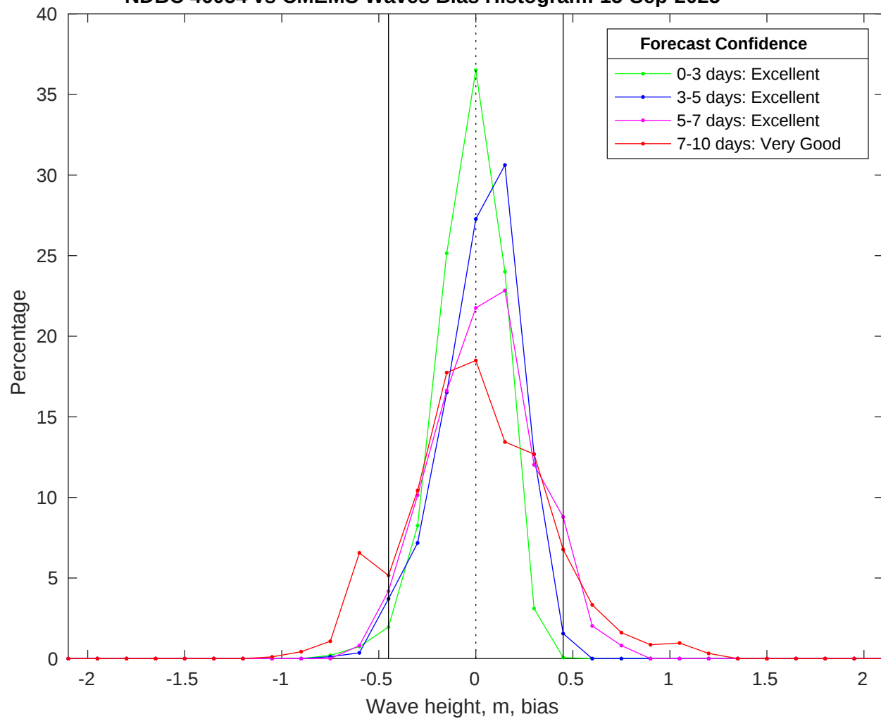
NDBC 46054 vs CMEMS Waves Bias Histogram: 15-Sep-2025
