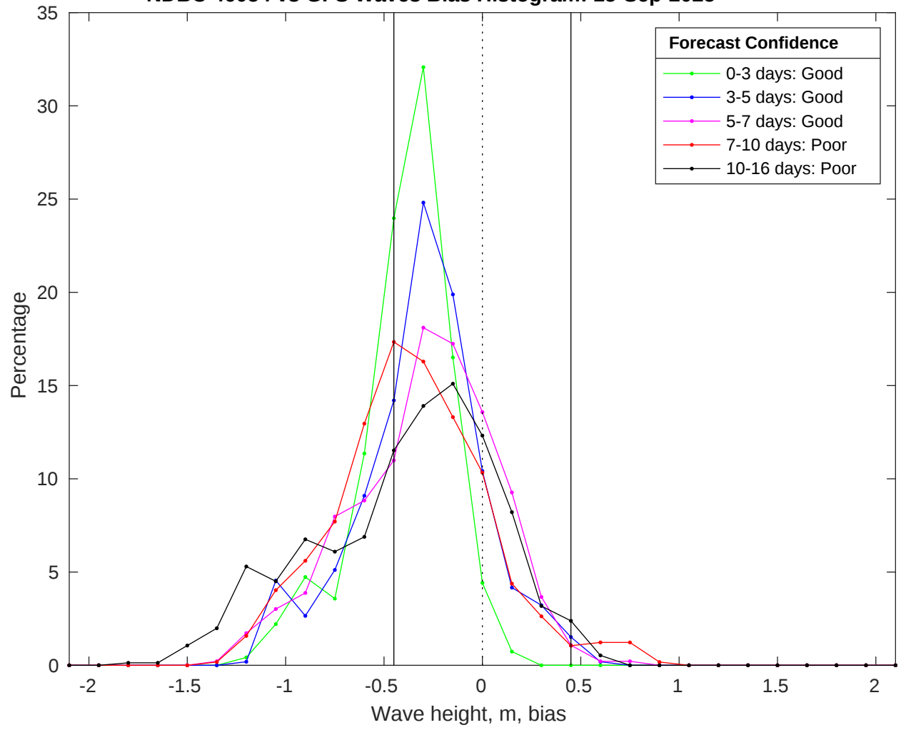
NDBC 46054 vs GFS Waves Bias Histogram: 15-Sep-2025
