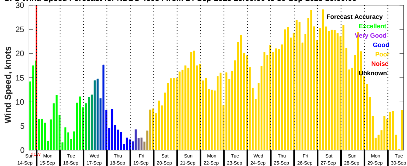
GFS Wind Speed Forecast for NDBC 46054 from 14-Sep-2025 16:00:00 to 30-Sep-2025 16:00:00
