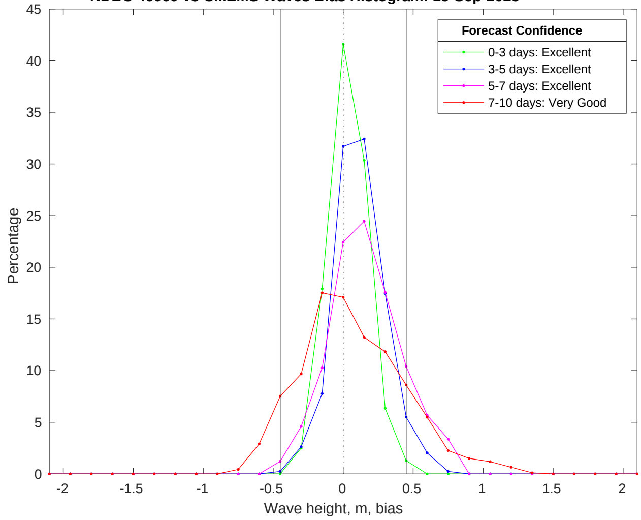
NDBC 46069 vs CMEMS Waves Bias Histogram: 15-Sep-2025
