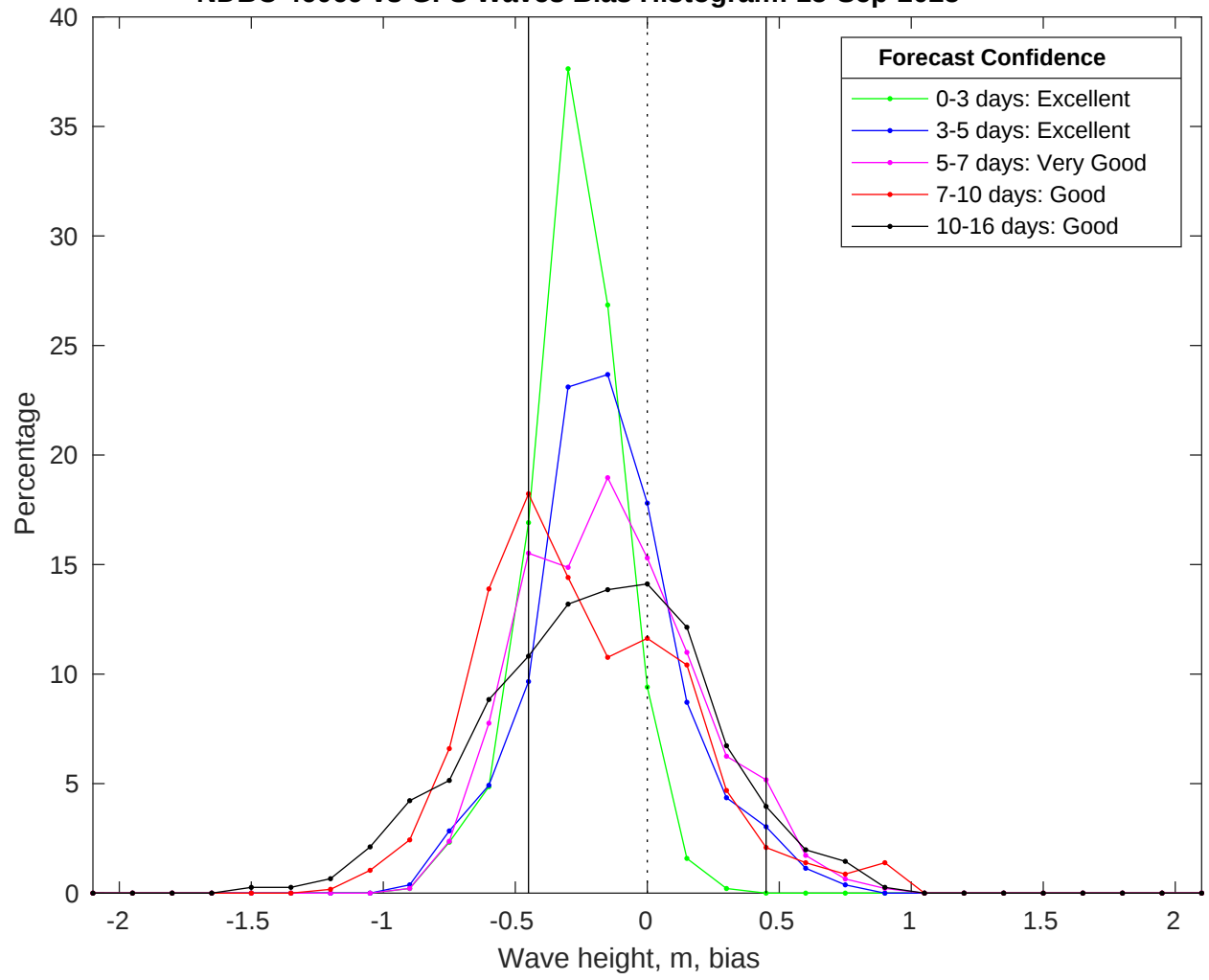
NDBC 46069 vs GFS Waves Bias Histogram: 15-Sep-2025
