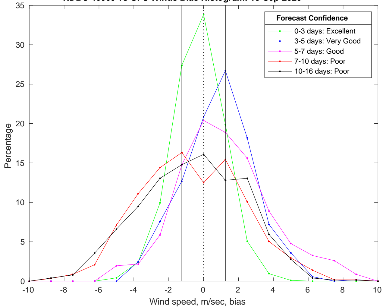
NDBC 46069 vs GFS Winds Bias Histogram: 15-Sep-2025
