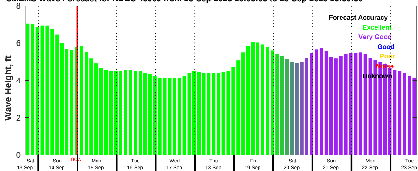
CMEMS Wave Forecast for NDBC 46069 from 13-Sep-2025 16:00:00 to 23-Sep-2025 16:00:00
