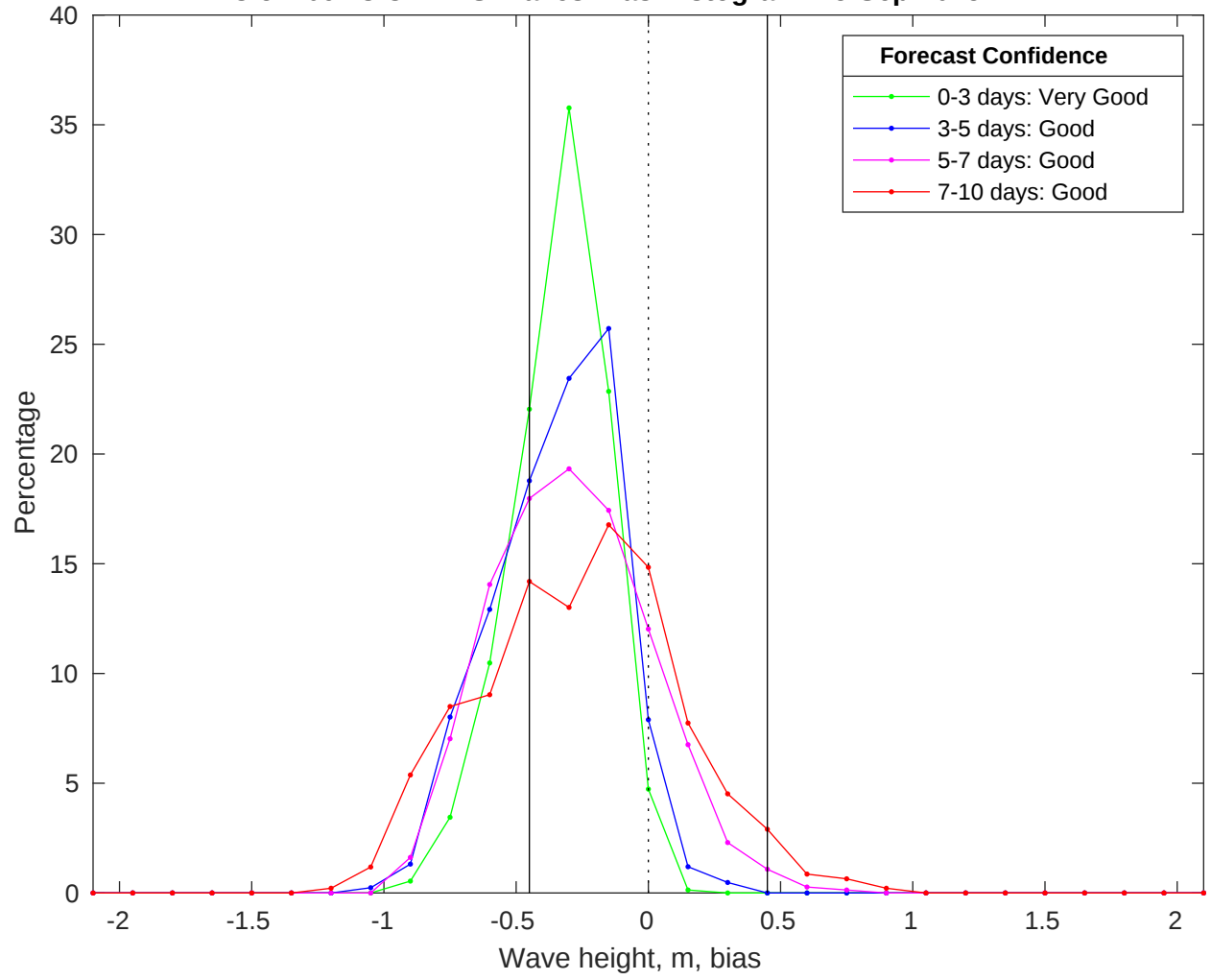
NDBC 51209 vs CMEMS Waves Bias Histogram: 15-Sep-2025
