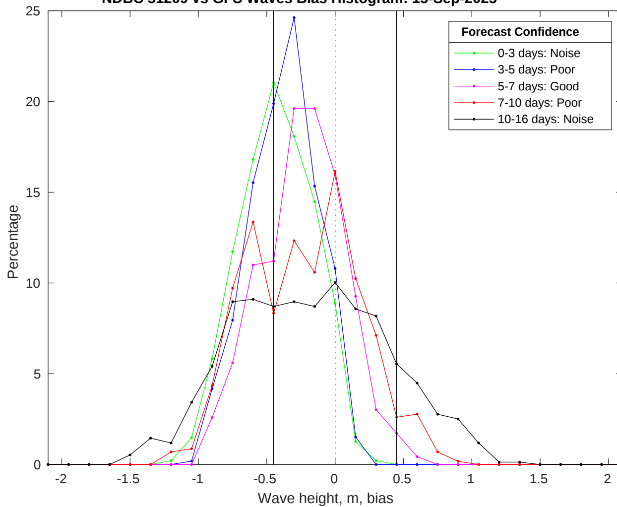
NDBC 51209 vs GFS Waves Bias Histogram: 15-Sep-2025
