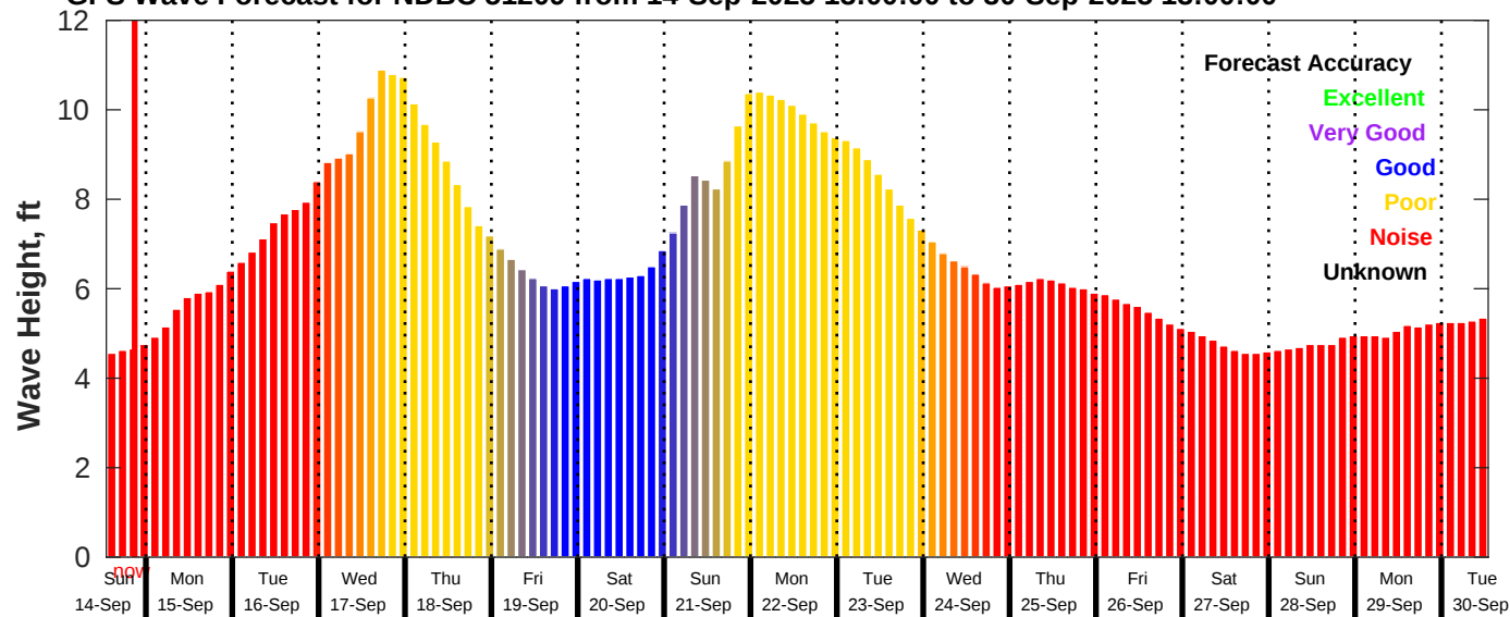
GFS Wave Forecast for NDBC 51209 from 14-Sep-2025 13:00:00 to 30-Sep-2025 13:00:00
