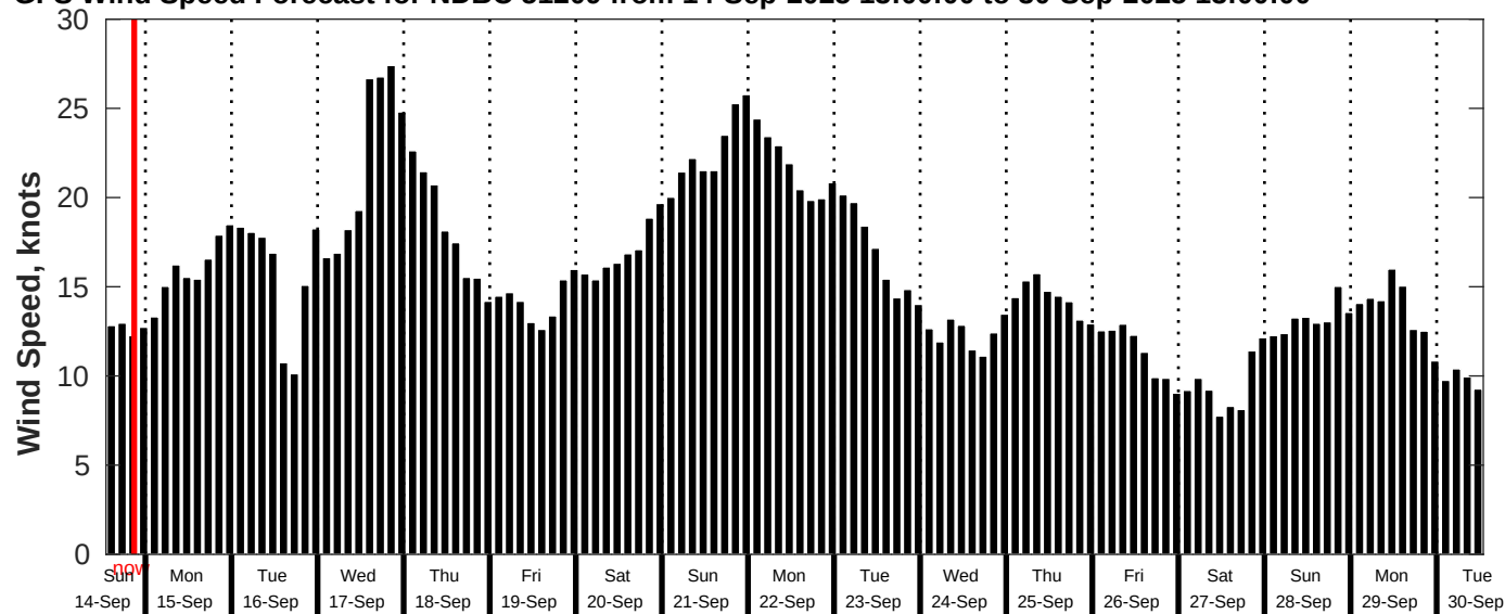
GFS Wind Speed Forecast for NDBC 51209 from 14-Sep-2025 13:00:00 to 30-Sep-2025 13:00:00
