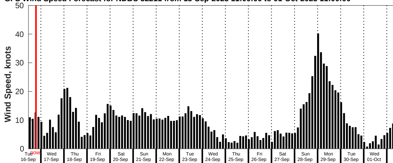
GFS Wind Speed Forecast for NDBC 52211 from 15-Sep-2025 11:00:00 to 01-Oct-2025 11:00:00
