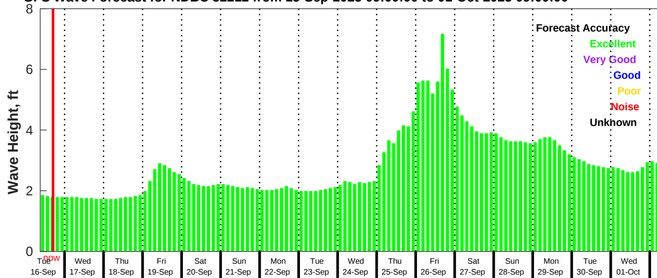
GFS Wave Forecast for NDBC 52212 from 15-Sep-2025 09:00:00 to 01-Oct-2025 09:00:00
