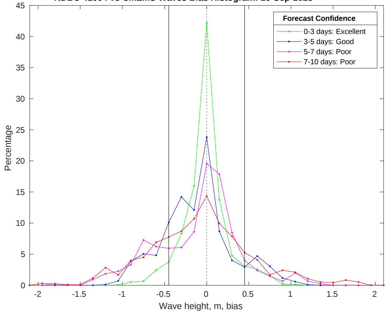
NDBC 41004 vs CMEMS Waves Bias Histogram: 16-Sep-2025
