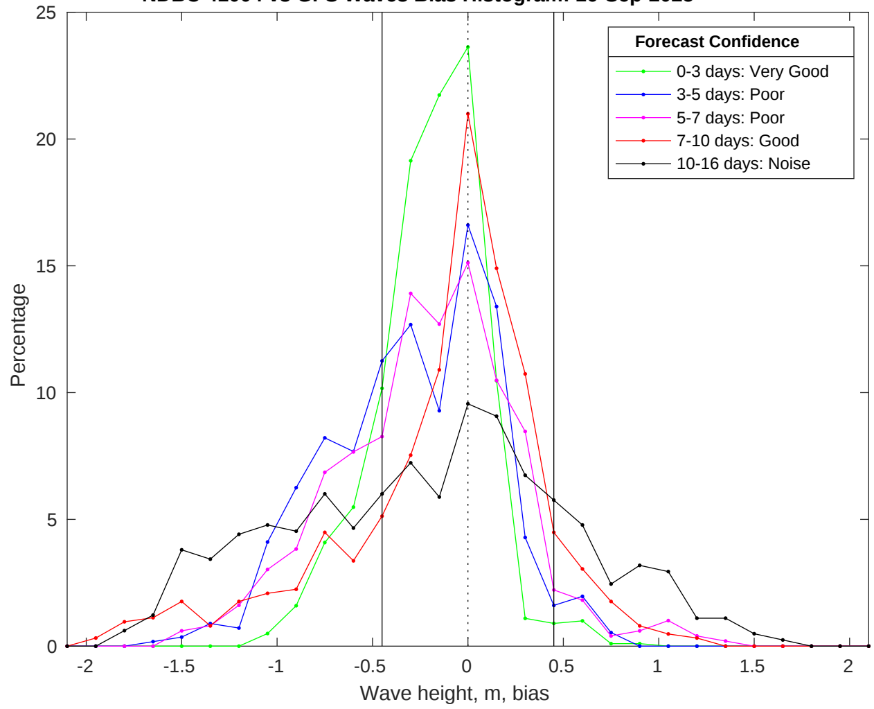
NDBC 41004 vs GFS Waves Bias Histogram: 16-Sep-2025
