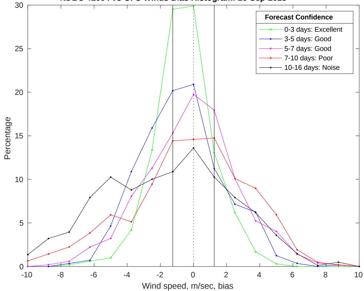
NDBC 41004 vs GFS Winds Bias Histogram: 16-Sep-2025
