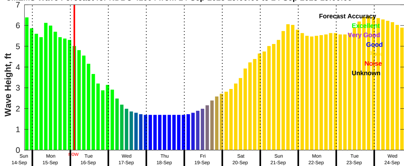
CMEMS Wave Forecast for NDBC 41004 from 14-Sep-2025 19:00:00 to 24-Sep-2025 19:00:00
