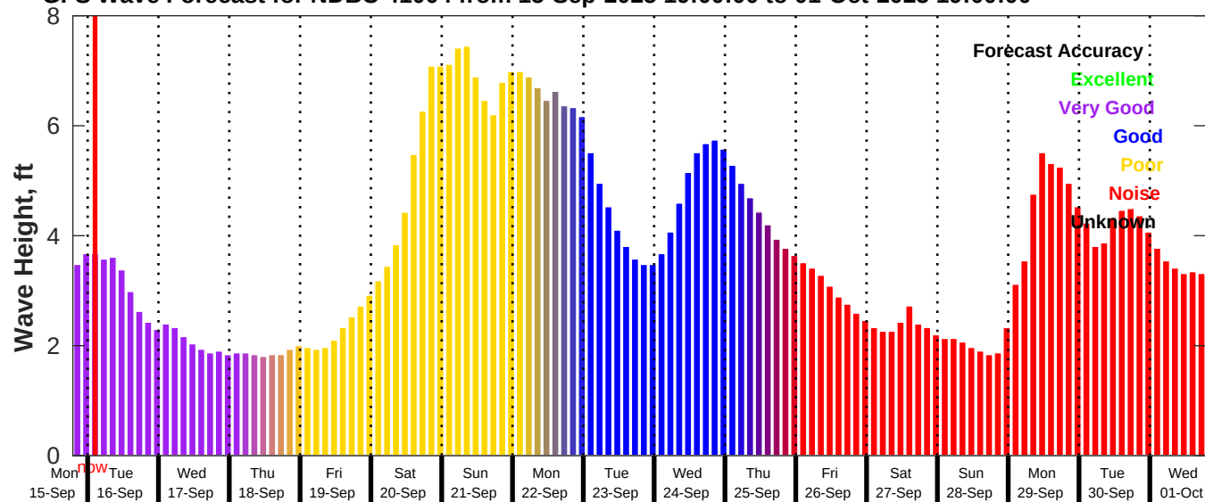
GFS Wave Forecast for NDBC 41004 from 15-Sep-2025 19:00:00 to 01-Oct-2025 19:00:00
