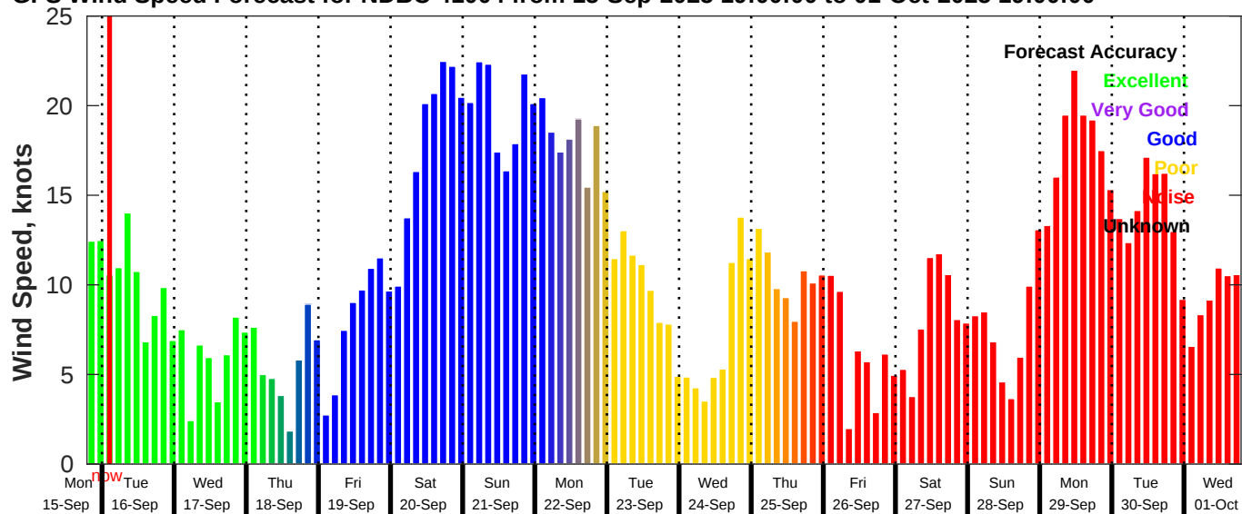
GFS Wind Speed Forecast for NDBC 41004 from 15-Sep-2025 19:00:00 to 01-Oct-2025 19:00:00
