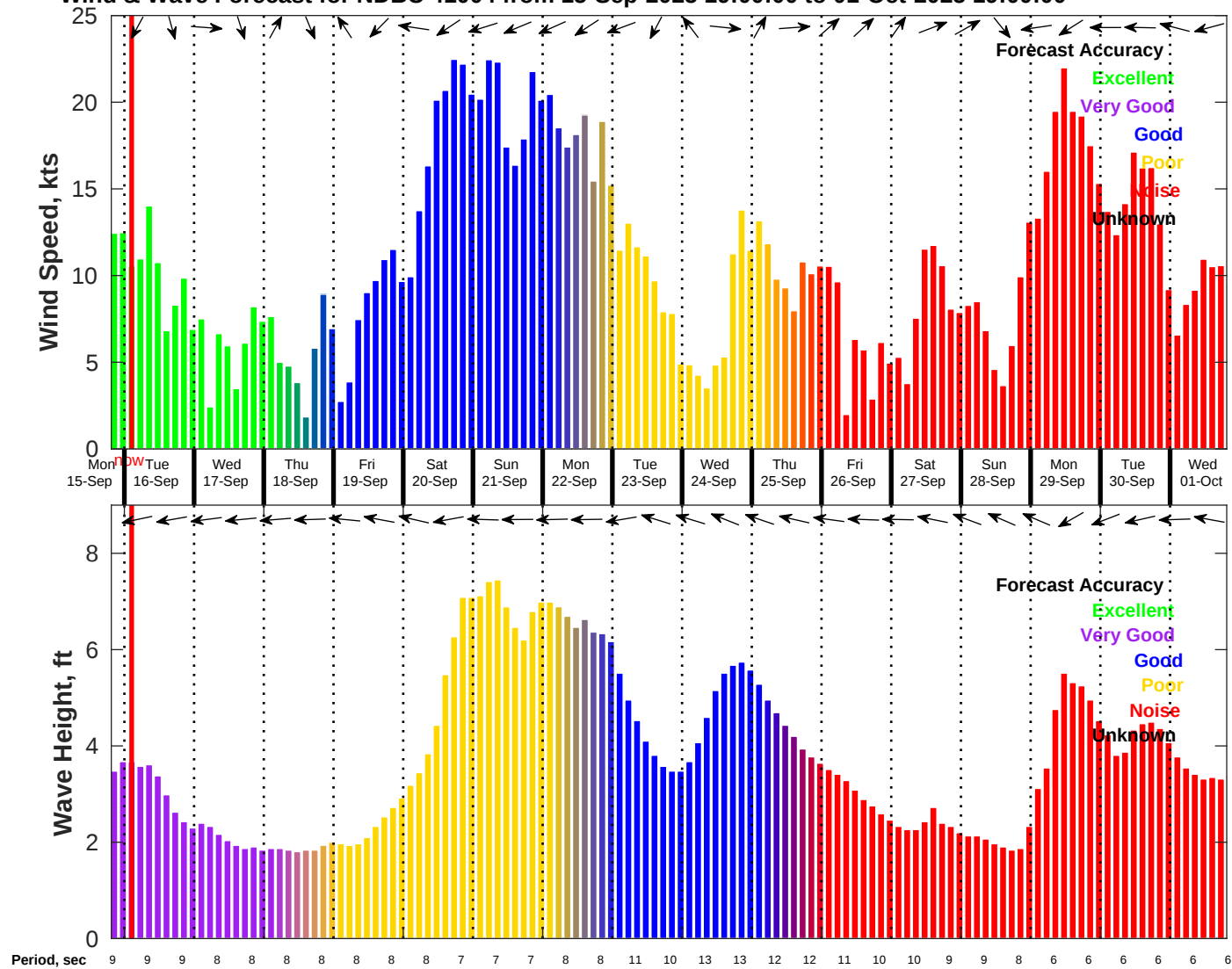
Wind & Wave Forecast for NDBC 41004 from 15-Sep-2025 19:00:00 to 01-Oct-2025 19:00:00
