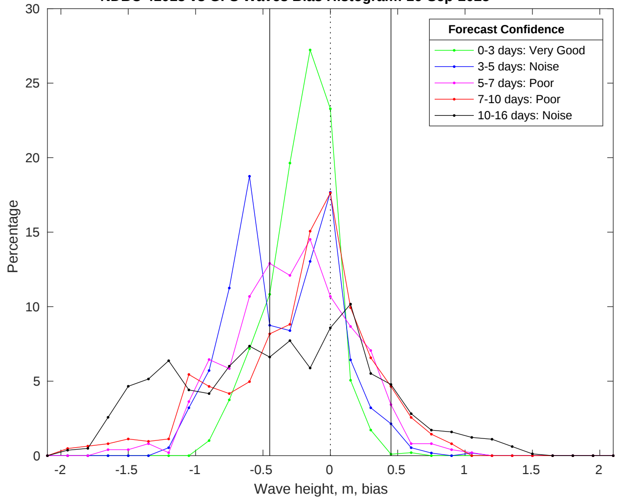
NDBC 41013 vs GFS Waves Bias Histogram: 16-Sep-2025
