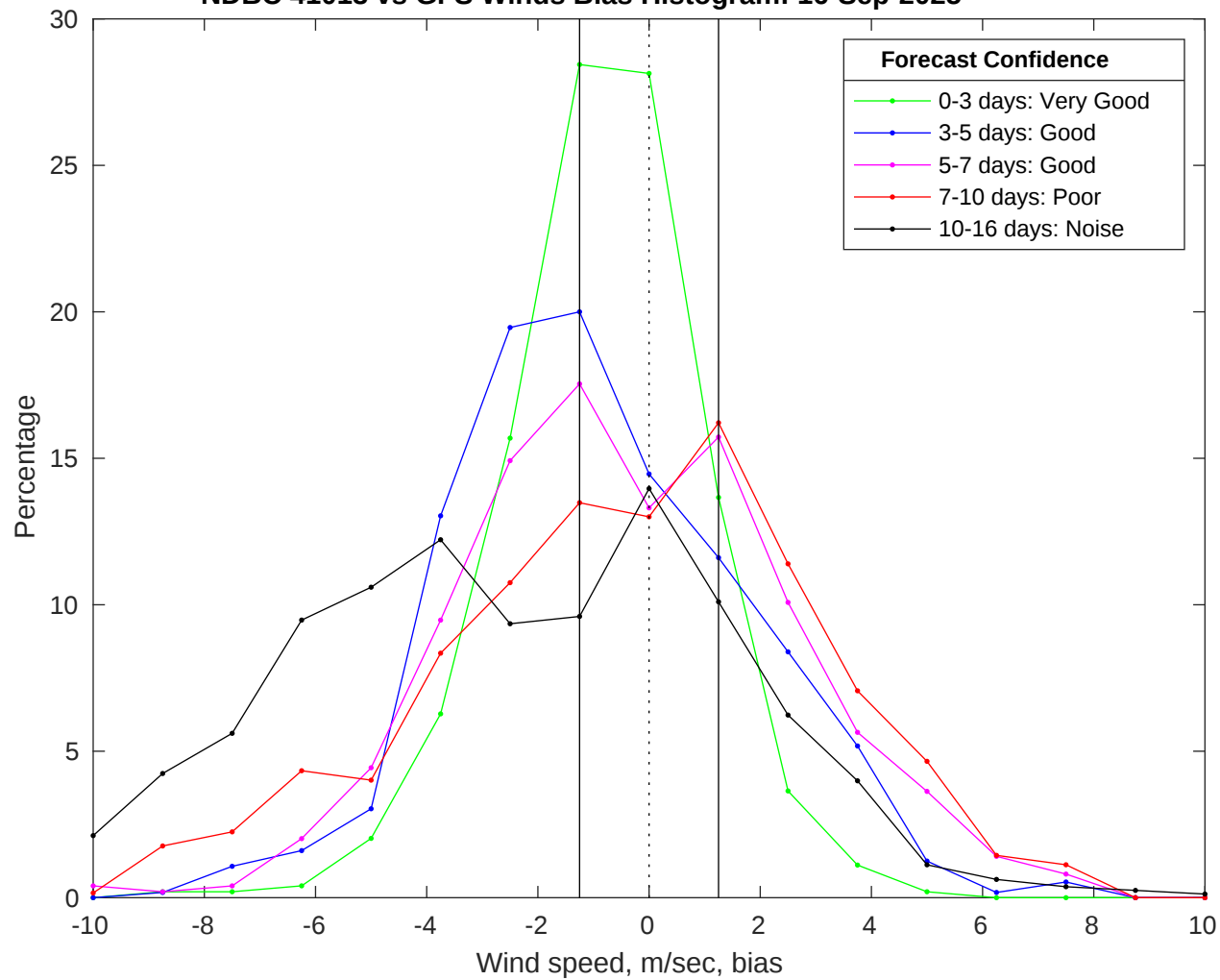
NDBC 41013 vs GFS Winds Bias Histogram: 16-Sep-2025
