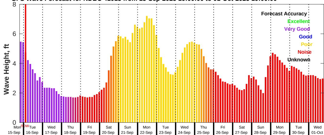
GFS Wave Forecast for NDBC 41013 from 15-Sep-2025 19:00:00 to 01-Oct-2025 19:00:00
