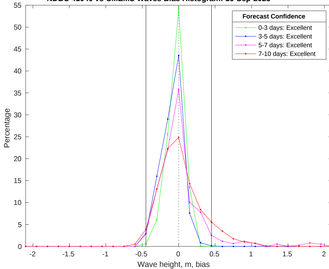
NDBC 41040 vs CMEMS Waves Bias Histogram: 16-Sep-2025
