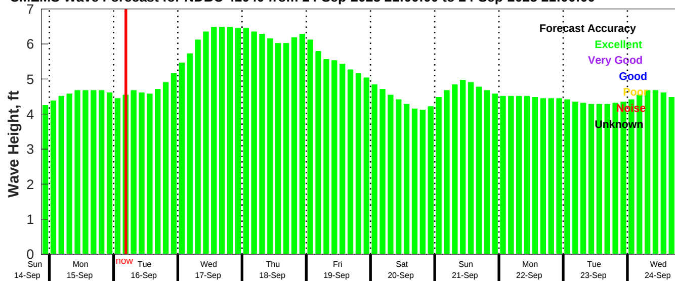
CMEMS Wave Forecast for NDBC 41040 from 14-Sep-2025 21:00:00 to 24-Sep-2025 21:00:00
