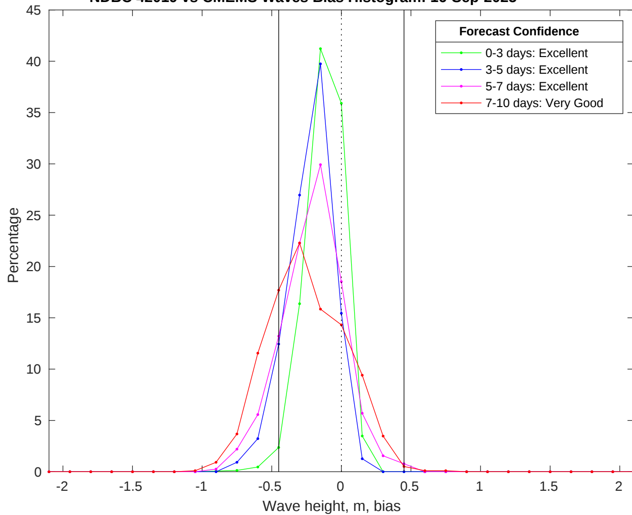
NDBC 42019 vs CMEMS Waves Bias Histogram: 16-Sep-2025
