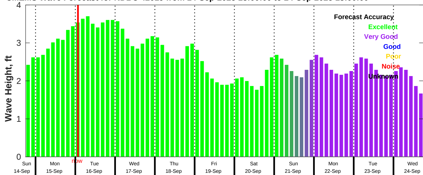
CMEMS Wave Forecast for NDBC 42019 from 14-Sep-2025 18:00:00 to 24-Sep-2025 18:00:00
