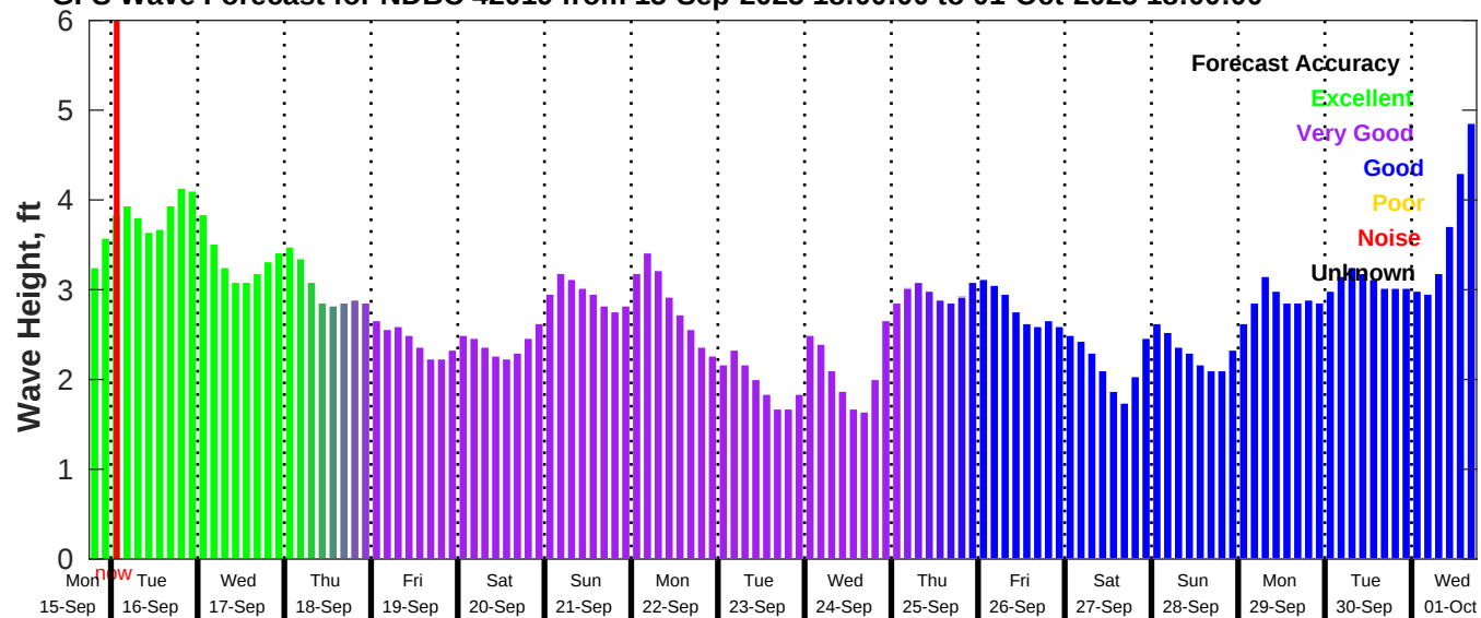
GFS Wave Forecast for NDBC 42019 from 15-Sep-2025 18:00:00 to 01-Oct-2025 18:00:00
