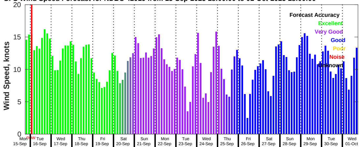
GFS Wind Speed Forecast for NDBC 42019 from 15-Sep-2025 18:00:00 to 01-Oct-2025 18:00:00
