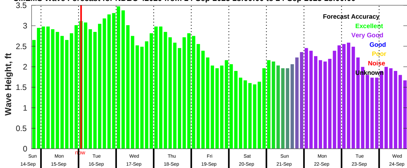
CMEMS Wave Forecast for NDBC 42020 from 14-Sep-2025 18:00:00 to 24-Sep-2025 18:00:00
