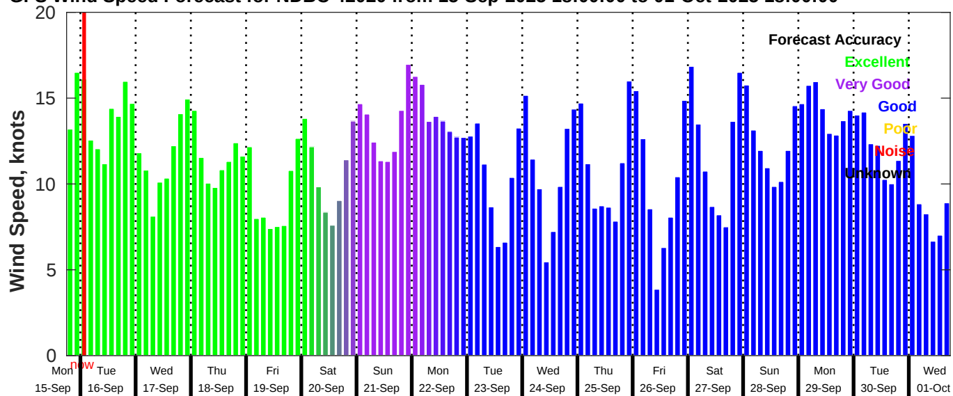
GFS Wind Speed Forecast for NDBC 42020 from 15-Sep-2025 18:00:00 to 01-Oct-2025 18:00:00
