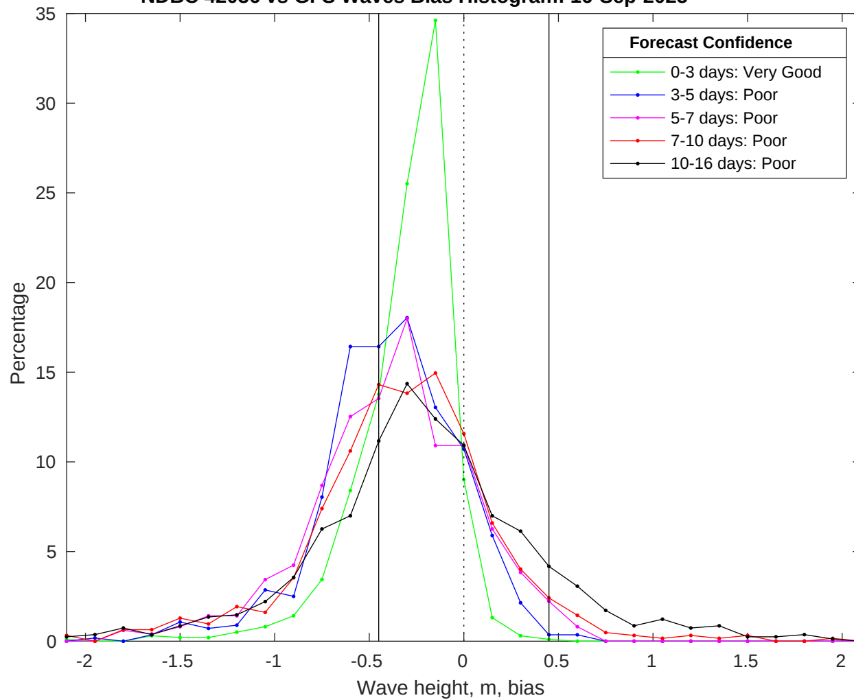
NDBC 42036 vs GFS Waves Bias Histogram: 16-Sep-2025
