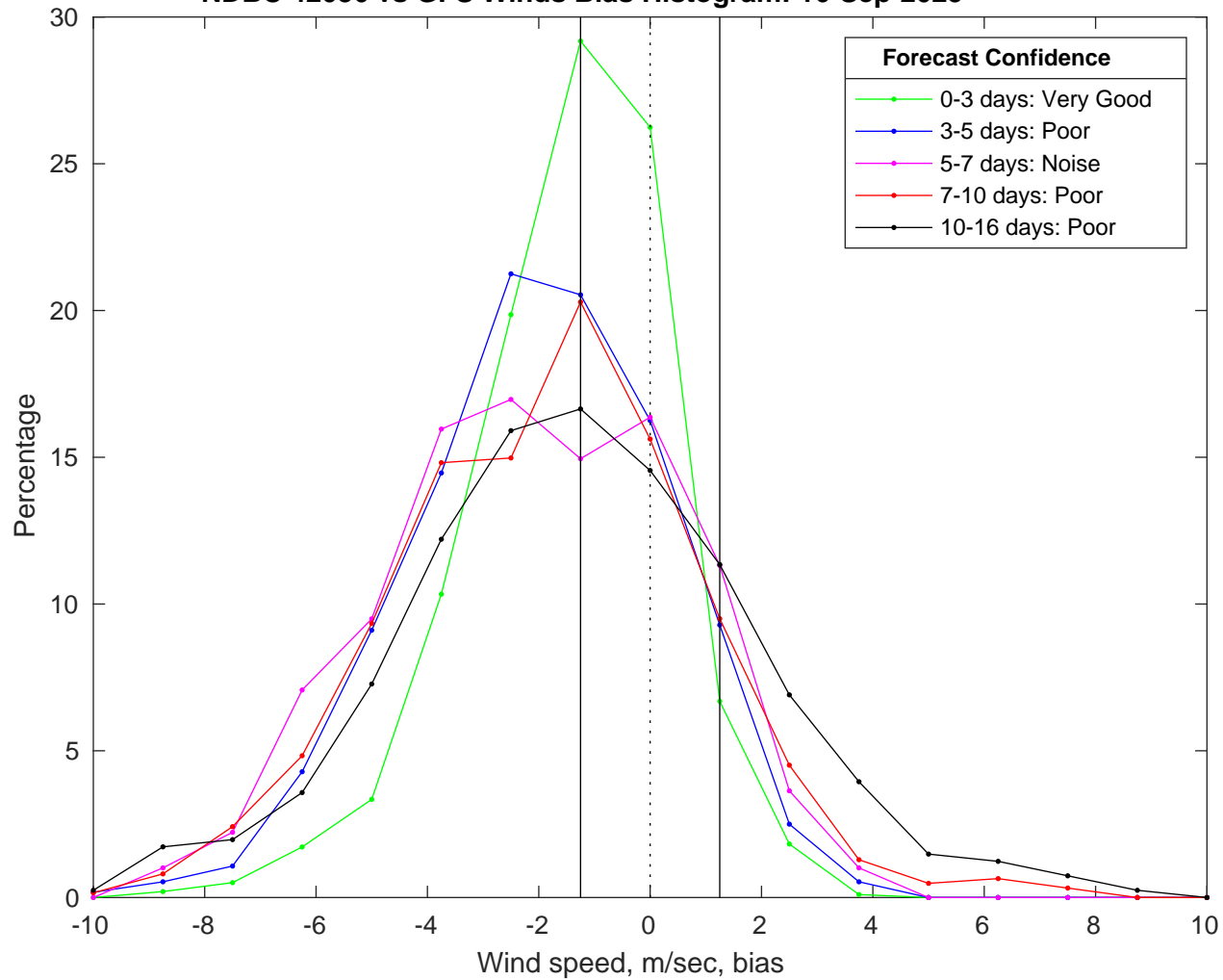
NDBC 42036 vs GFS Winds Bias Histogram: 16-Sep-2025
